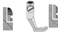
Piedino anteriore Front foot 067 2207 3/01
