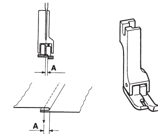
Narrow right compensating foot
