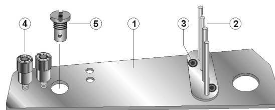
Piastra vibrante cpl. Vibrating plate 069 001449 4
